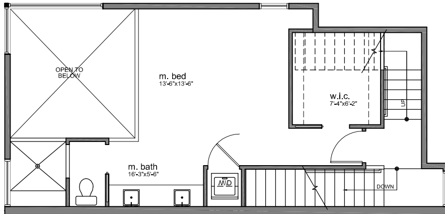
ne unit - 3rd floor plan
