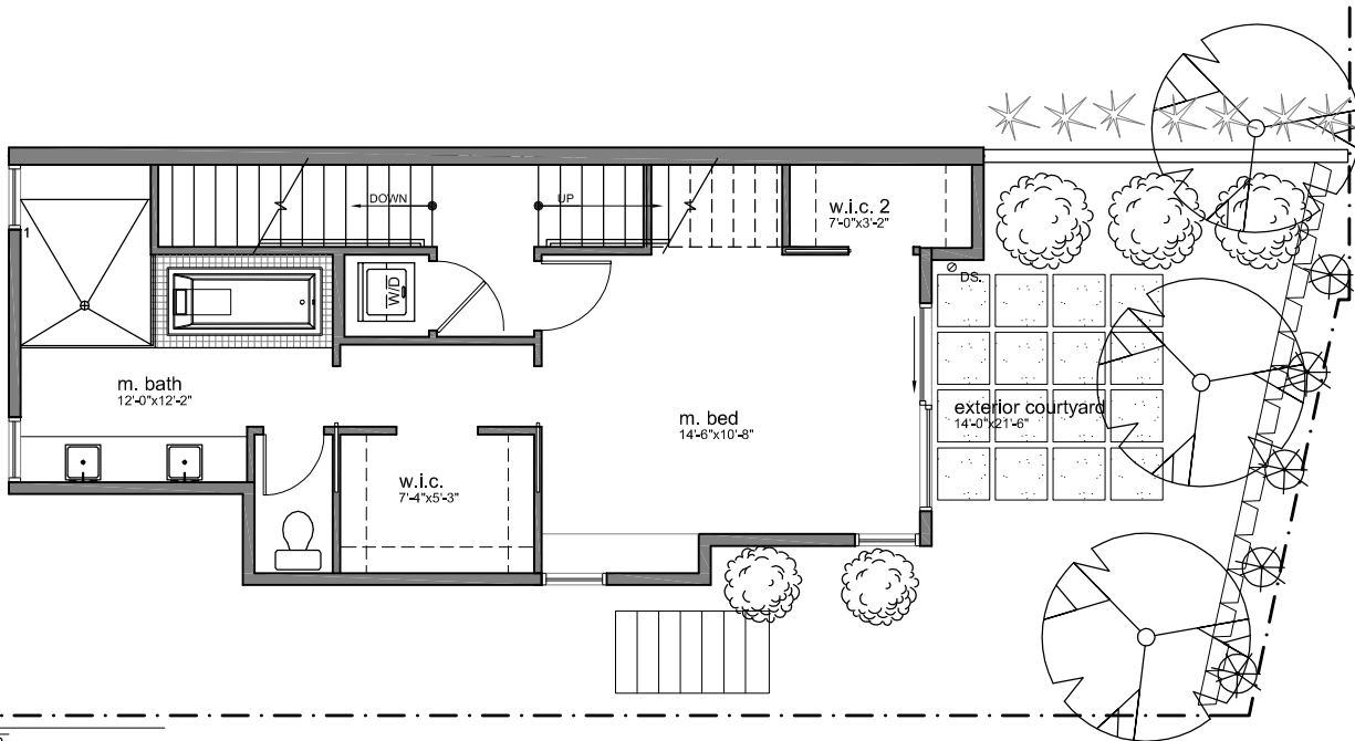
se unit - 2nd floor plan
