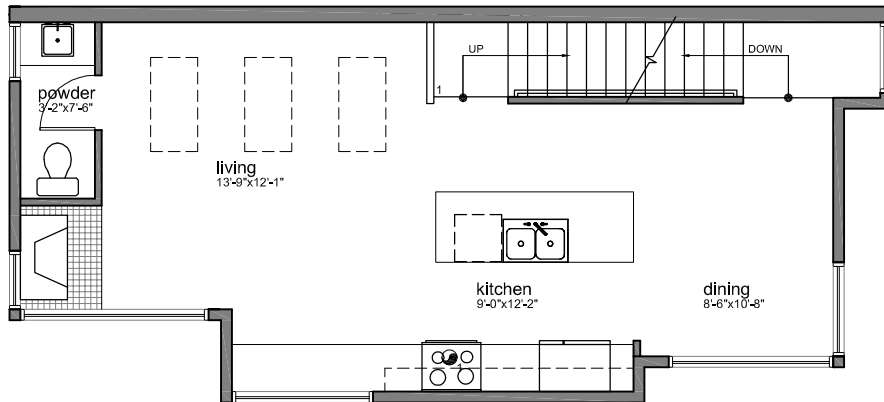
se unit - 3rd floor plan
