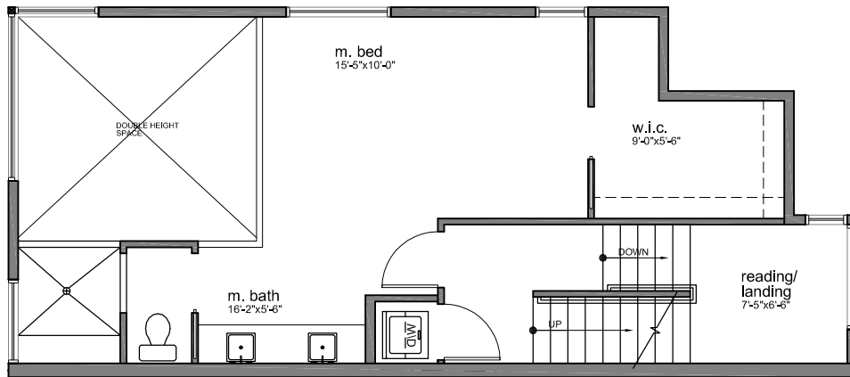
nw unit - 3rd floor plan
